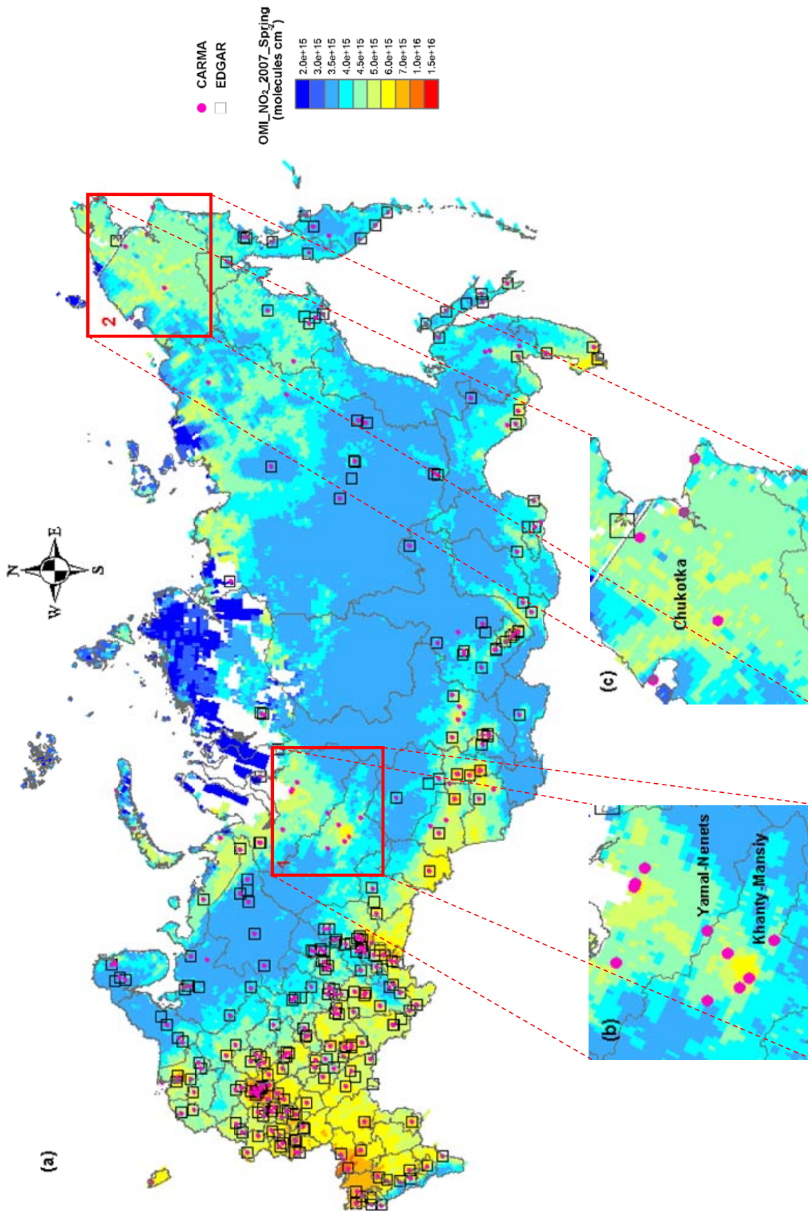
Fig. 3. 2007 Springtime average OMI NO 2 (0.25° × 0.25°) column concentrations (molecules/cm 2 ) over (a) the whole Russian country and two sub-regions, i.e., (b) Sub-region 1: the Urals Federal District and (c) Sub-region 2: Chukotka Autonomous Okrug. Pink dots and black squares represent the locations of thermal power plants from CARMA and EDGAR v4.2 in 2007, respectively. The CARMA power plant data is at precise locations while the EDGAR is gridded with a spatial resolution of 0.1° × 0.1°.
