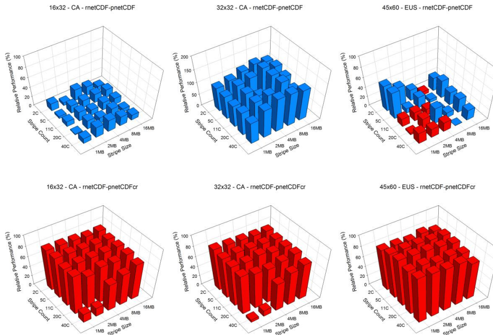
Figure 10. Relative performance of pnetCDF and pnetCDFcr with respect to rnetCDF in a large number of processors scenario on Kraken. Red color denotes positive value in relative performance while blue color denotes negative value in relative performance.
