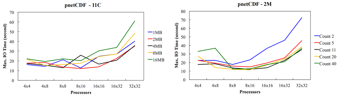
Figure 9. The impact of stripe count and size on parallel netCDF I/O performance on the CONUS domain. Left: various stripe sizes with fixed 11-stripe counts. Right: various stripe counts with fixed 2 MB stripe size.
