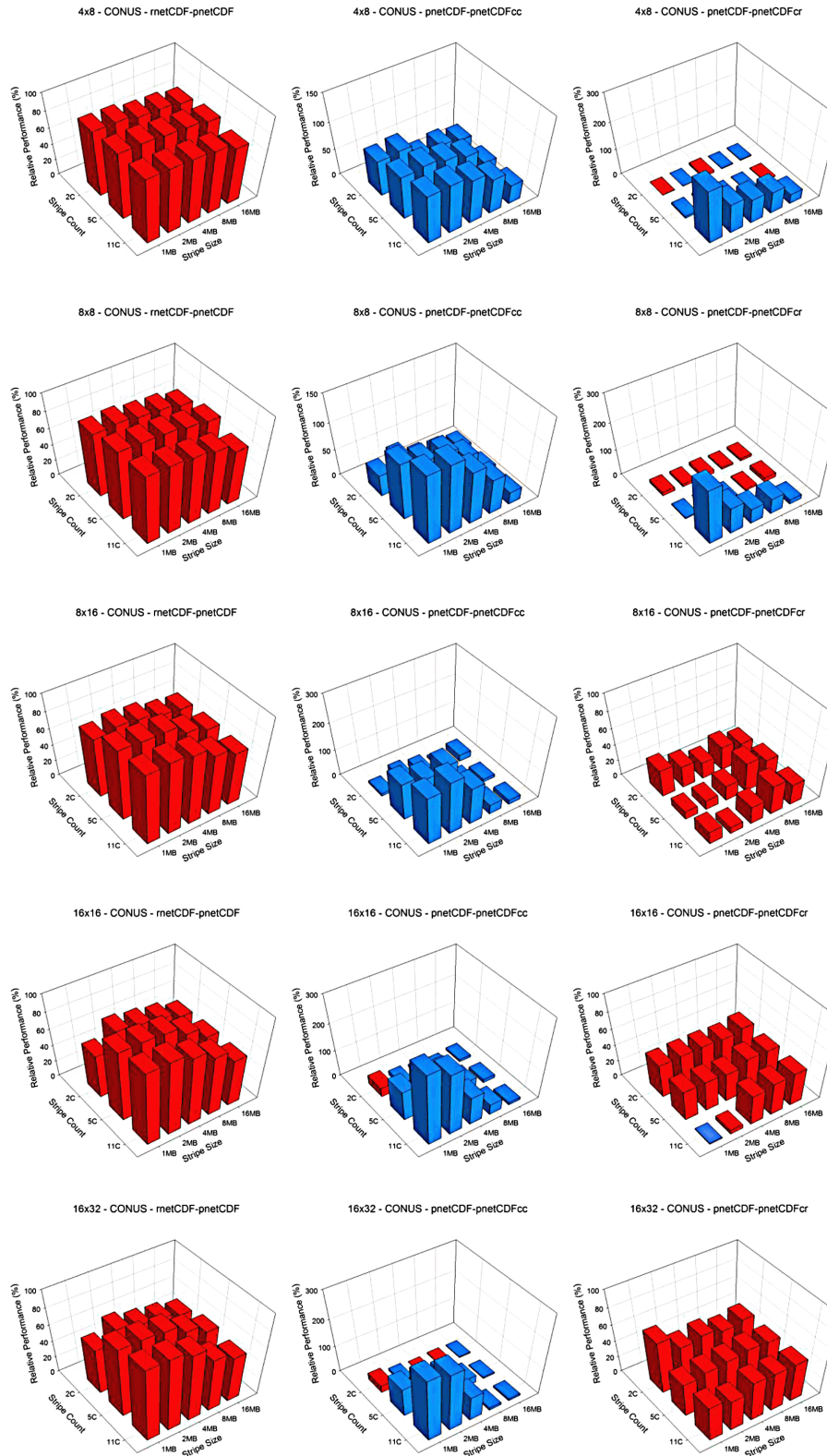
Figure 8. Relative I/O performance of pnetCDF to metCDF, and pnetCDFcc and pnetCDFcr to pnetCDF on the CONUS domain with 4 × 8, 8 × 8, 8 × 16, 16 × 16, and 16 × 32 processor configurations from Edison. Red color denotes positive value in relative performance while blue color denotes negative value in relative performance.
