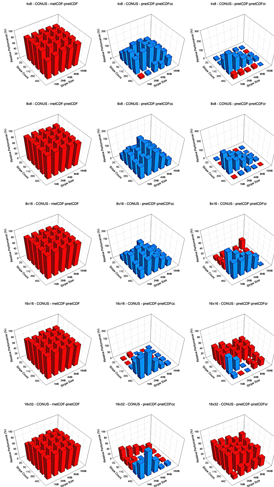
Figure 7. Relative I/O performance of pnetCDF to metCDF, and pnetCDFcc and pnetCDFcr to pnetCDF on the CONUS domain with 4 \times 8 , 8 \times 8 , 8 \times 16 , 16 \times 16 , and 16 \times 32 processor configurations from Kraken. Red color denotes positive value in relative performance while blue color denotes negative value in relative performance.
