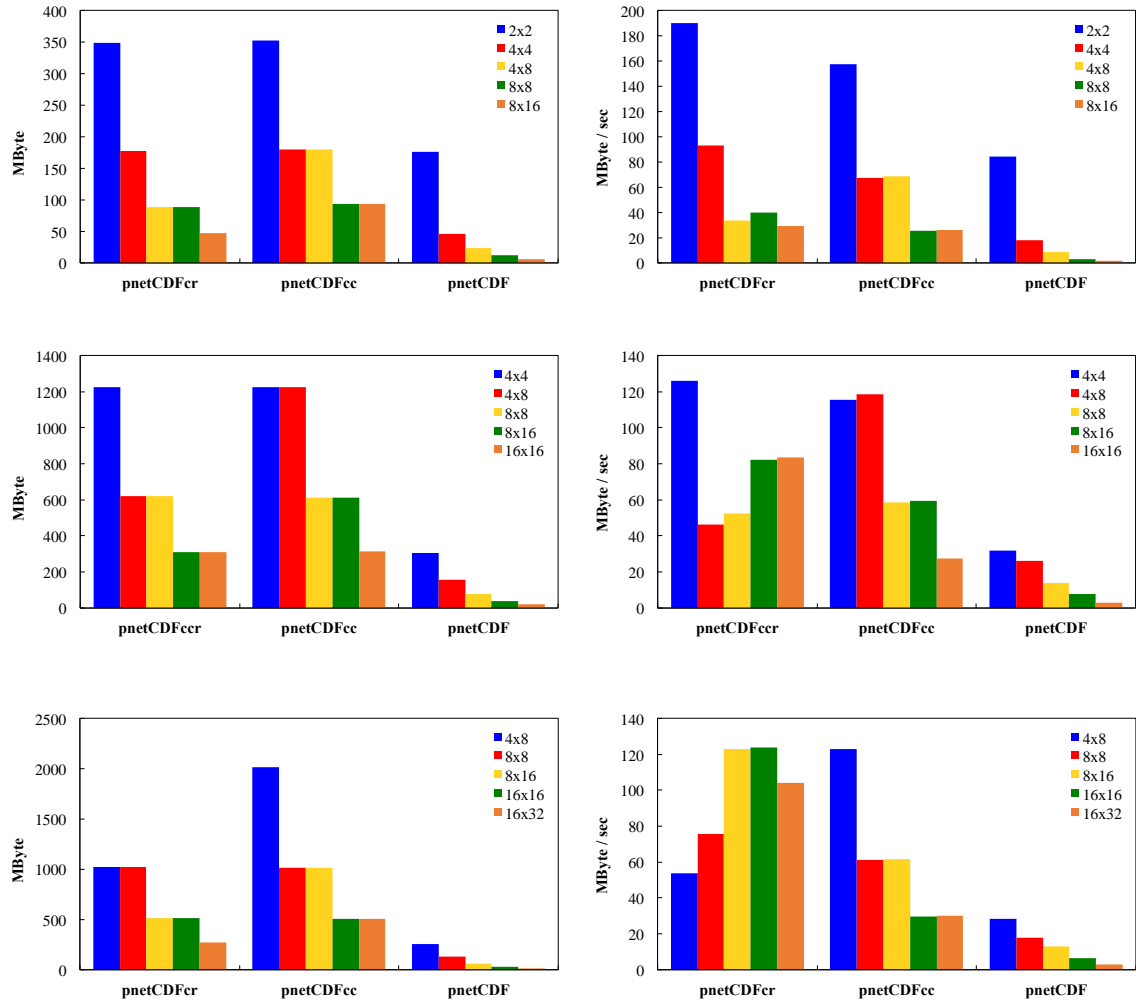
Figure 11. The maximum data size (left panel) and I/O rate (right panel) among all I/O processors in the CA (top), EUS (middle) and CONUS domains (bottom), respectively, in the pseudo-code experiment running on Edison.
