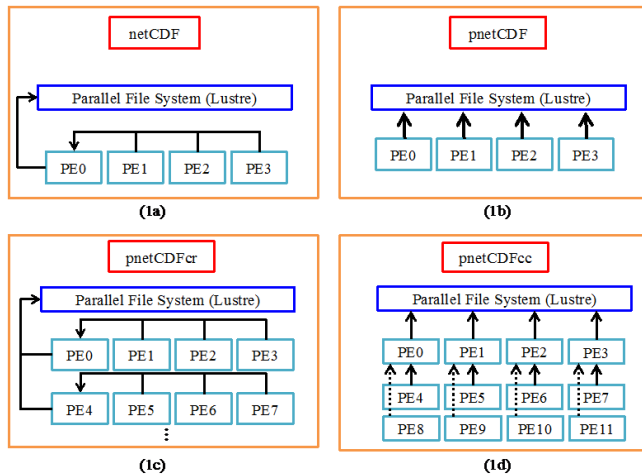
Figure 1. Conceptual diagrams of four I/O modules: serial I/O used in current CMAQ with netCDF data format (a), straight pnetCDF implementation (b), with data aggregation along row dimension and then use of pnetCDF (c), and with data aggregation along column dimension and then use of pnetCDF (d). PE denotes a processor. Arrows show the direction of data movement.
