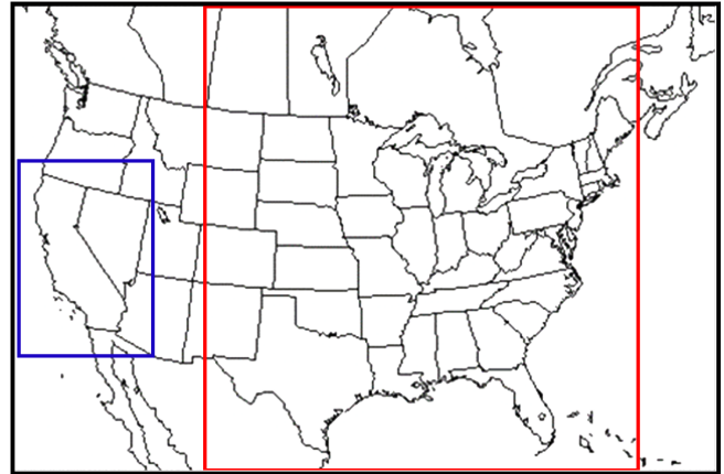
Figure 2. Regional representation of the CA (blue box), EUS (red box) and CONUS domains.
