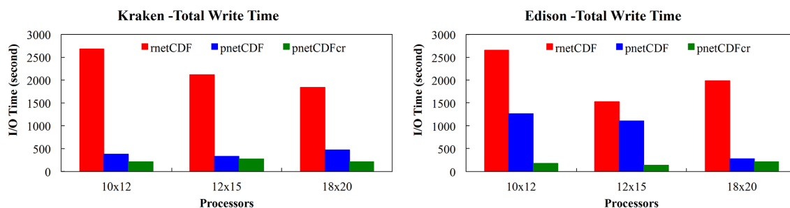
Figure 12. Total write time in a 1-day CMAQ simulation by different I/O approaches on a 4 km EUS domain with stripe size of 2 MB and stripe count of 11 (Kraken left and Edison right).
