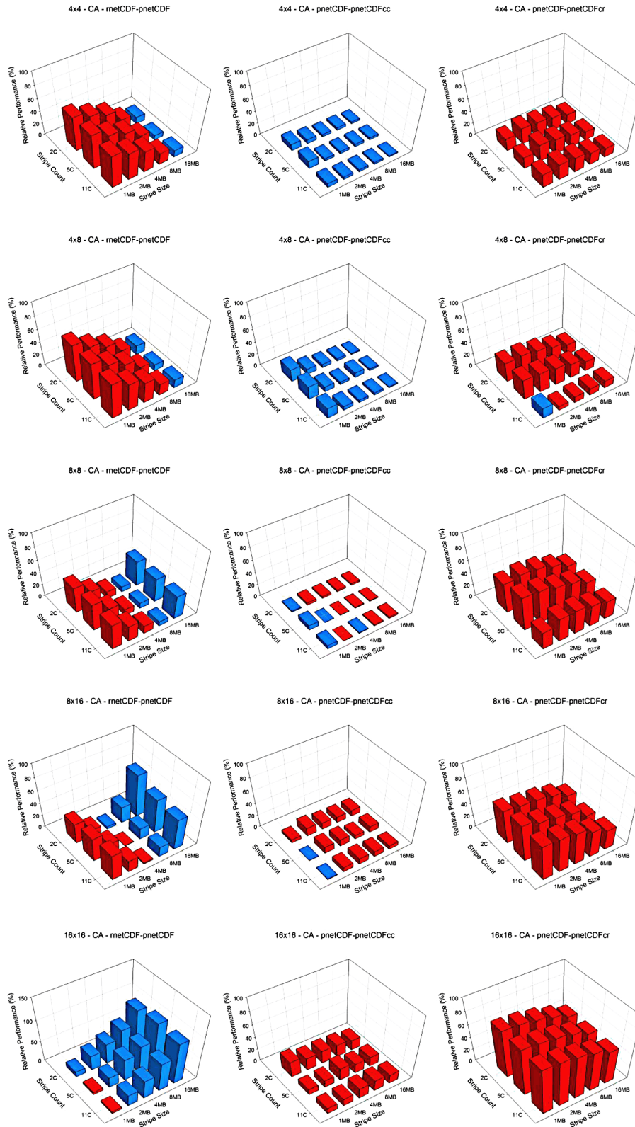
Figure 4. Relative I/O performance of pnetCDF to metCDF, and pnetCDFcc and pnetCDFcr to pnetCDF on the CA domain with 4 \times 4 , 4 \times 8 , 8 \times 8 , 8 \times 16 , and 16 \times 16 processor configurations from Edison. Red color denotes positive value in relative performance while blue color denotes negative value in relative performance.
