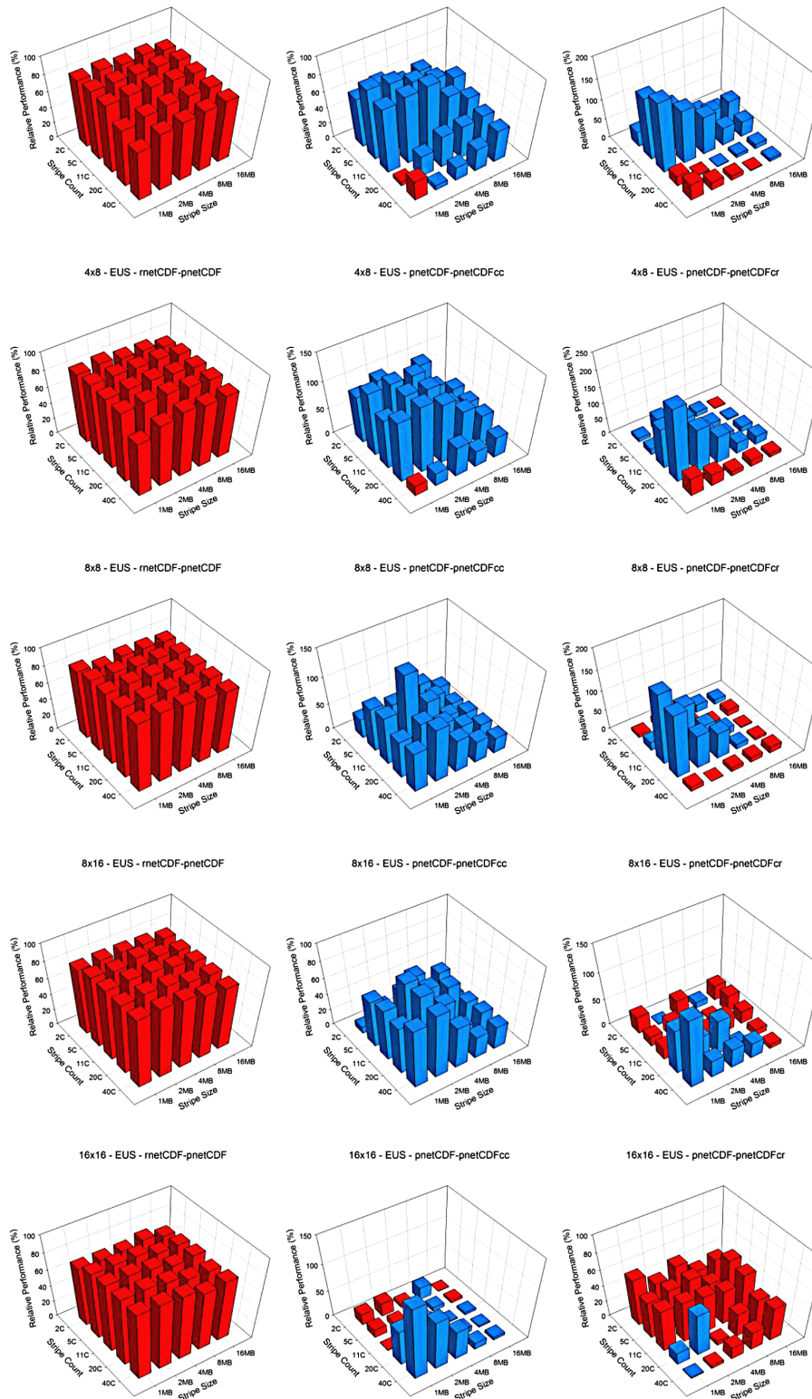
Figure 5. Relative I/O performance of pnetCDF to metCDF, and pnetCDFcc and pnetCDFcr to pnetCDF on the EUS domain with 4 \times 4 , 4 \times 8 , 8 \times 8 , 8 \times 16 , and 16 \times 16 processor configurations from Kraken. Red color denotes positive value in relative performance while blue color denotes negative value in relative performance.
