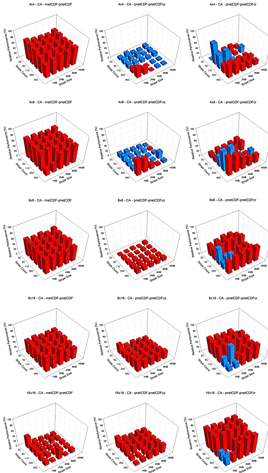
Figure 3. Relative I/O performance of pnetCDF to metCDF, and pnetCDFcc and pnetCDFcr to pnetCDF on the CA domain with 4 \times 4 , 4 \times 8 , 8 \times 8 , 8 \times 16 , and 16 \times 16 processor configurations from Kraken. Red color denotes positive value in relative performance while blue color denotes negative value in relative performance.
